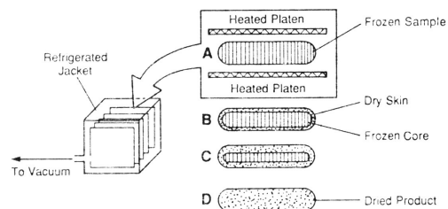
Figure 11.2-2. A freeze dryer. This type of equipment, which is often used for food, dries the solid via the sequence A → D shown on the right (After King and Clark, ibid. )
