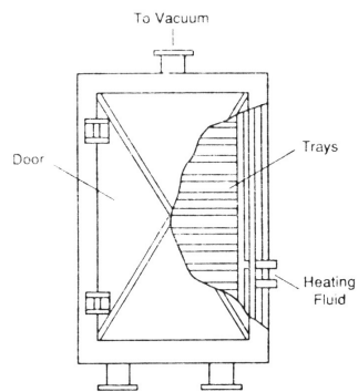
Figure 11.2-1. A tray dryer. Units like this are simple, flexible, and common, but can imply high labor costs (After King and Clark, AIChE Symposium Series 205 , 1977).
