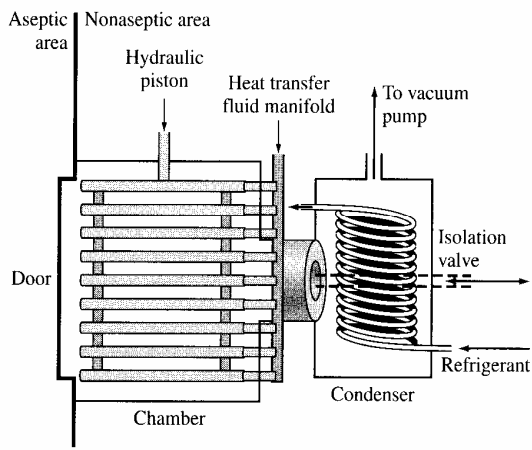
Figure 10.7 Pharmaceutical freeze dryer.
