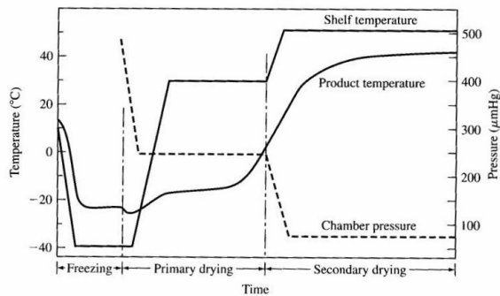
Figure 10.9 Process variables during the freeze-drying cycle.
